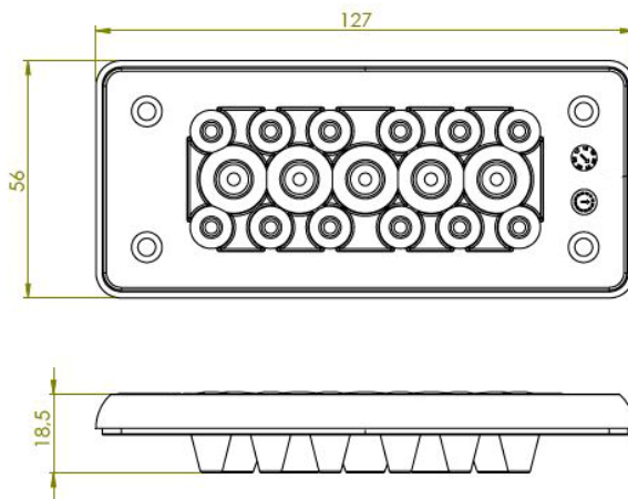
Dimensions of MH16
