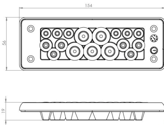
Dimensions of MH24
