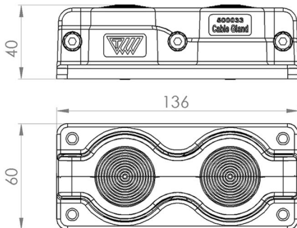
Dimensions of SCG 2x3-35
