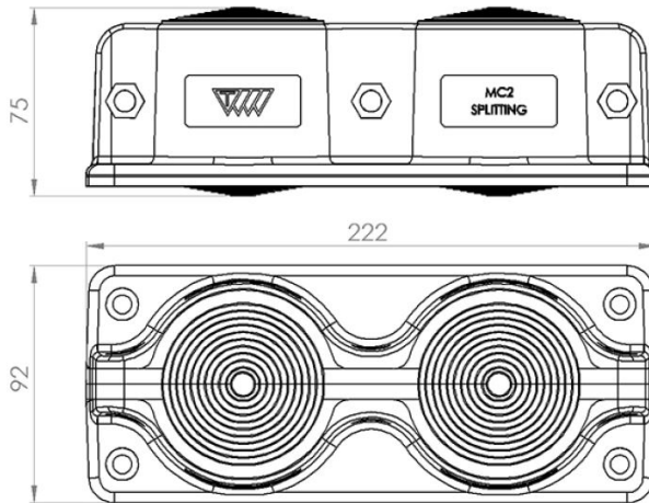
Dimensions of MC 2/10 + MC 2/18
