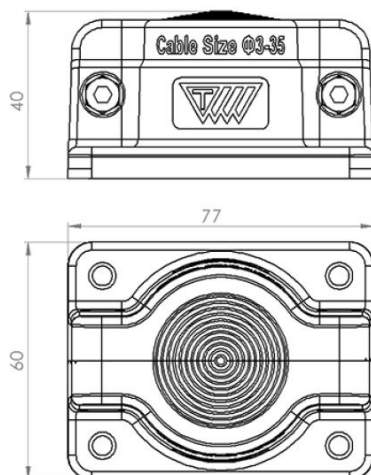
Dimensions of SCG 1x3-35
