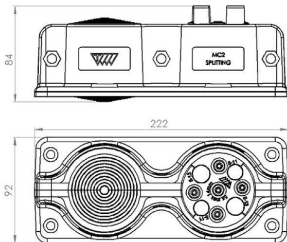
Dimensions of MC 2/10 + MC 2/18
